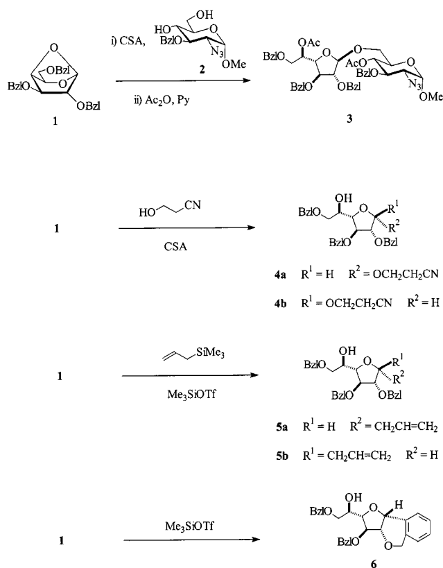
Scheme 1. Regioselective ring opening of the benzylated bicyclic compound 1 by various nucleophiles under acidic conditions
